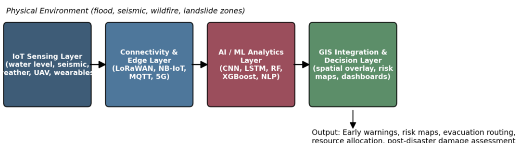
Figure 1: Conceptual four-layer architecture for AI-IoT-GIS integrated disaster risk management, synthesised from the reviewed literature
